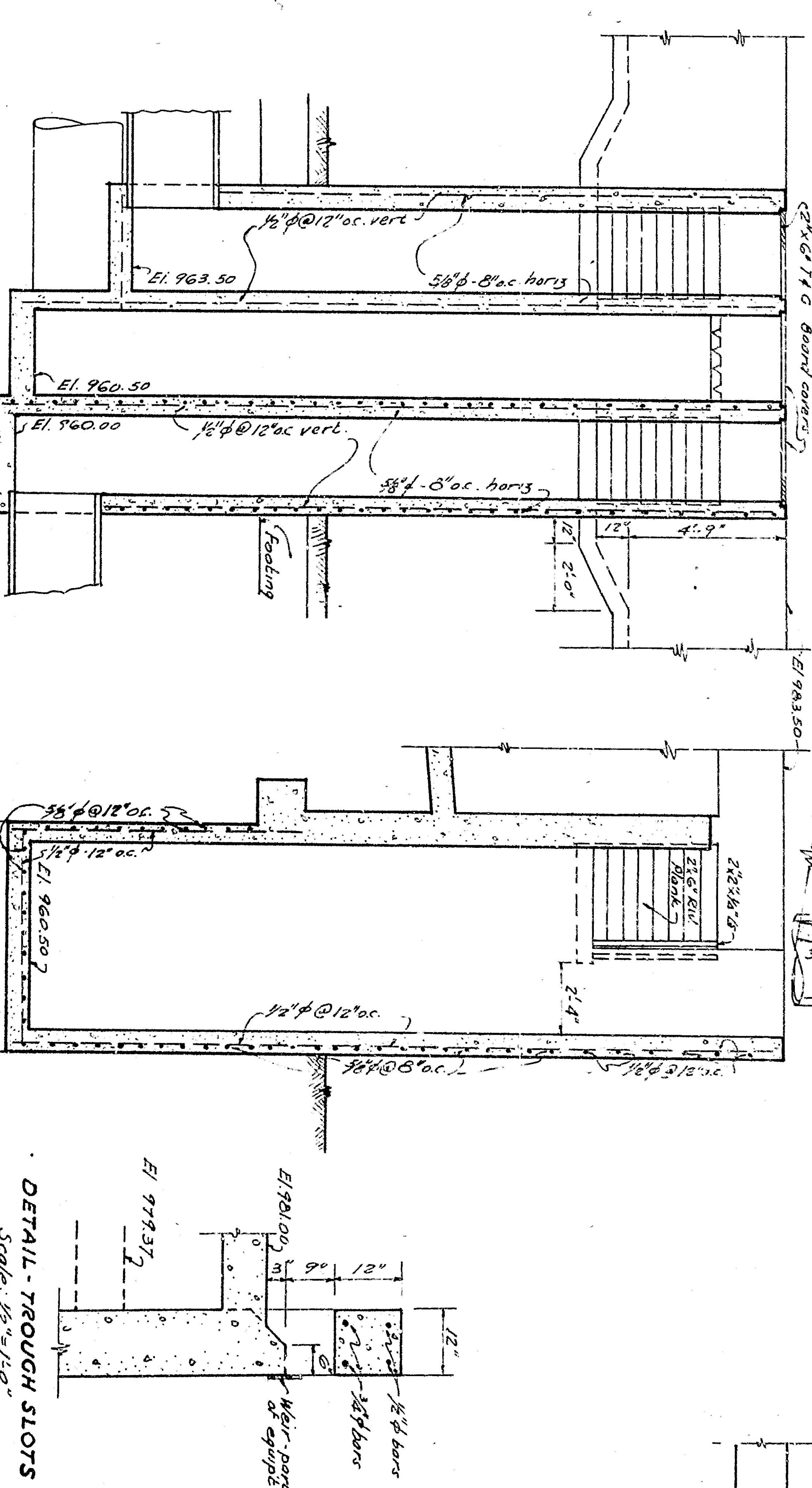
SECTIONS: PLAN - OUTLET BOX Scale: 1/4" = 1'-0"
